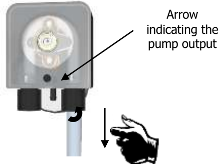
Step 14 Screw the cap with the PE tubing (white) onto the pump.
