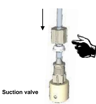
Step 15 Unscrew the cap and thread the clear tube through it.
