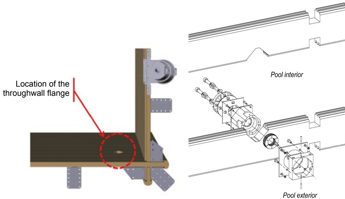
Figure 27 – Position of the throughwall flange
