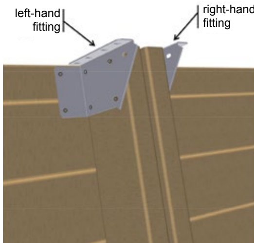
Figure 19 – Mounting the fittings on top of the supporting brace
