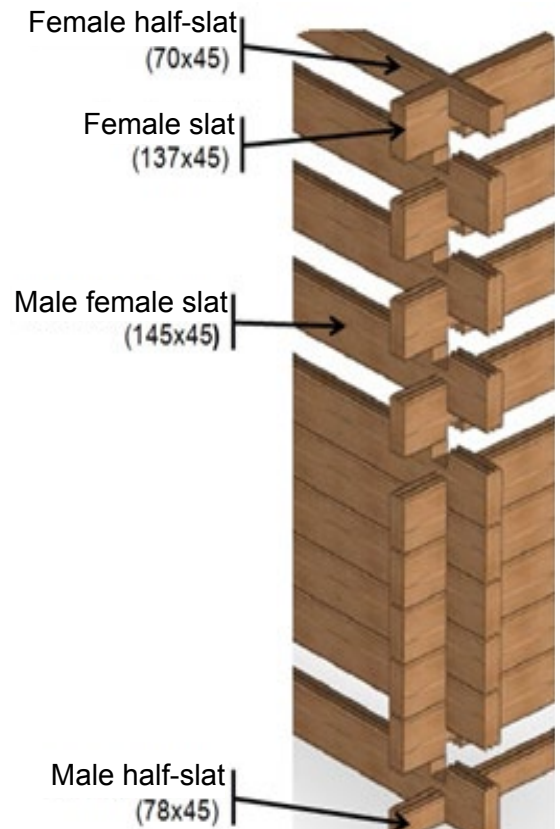
Figure 60 – Slotting together the wooden slats
