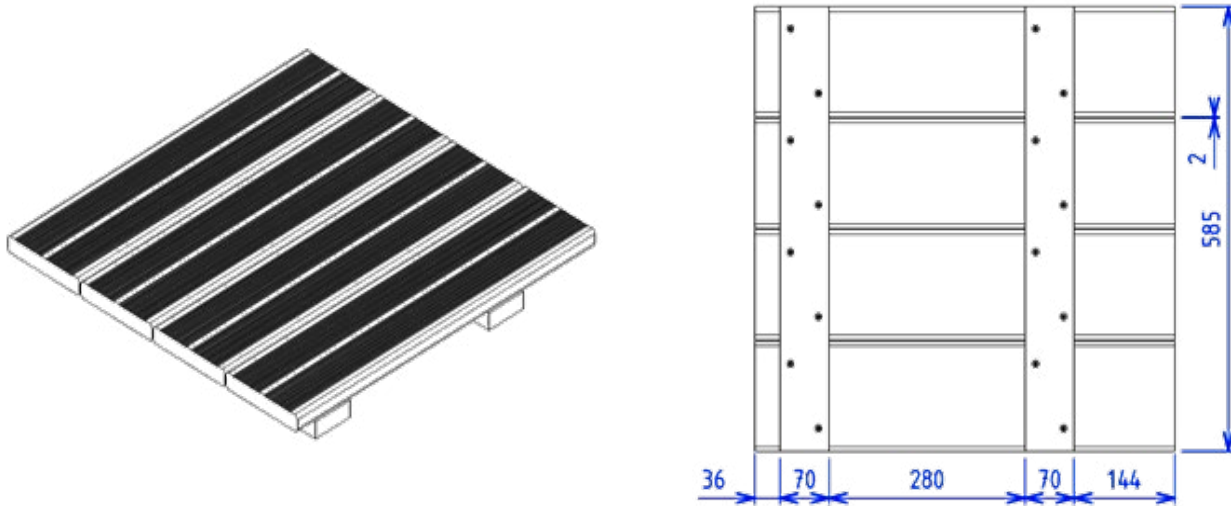
Figure 52 – Assembling the duckboarding
