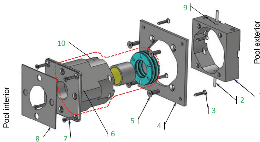
Figure 28 – Mounting the throughwall flange
