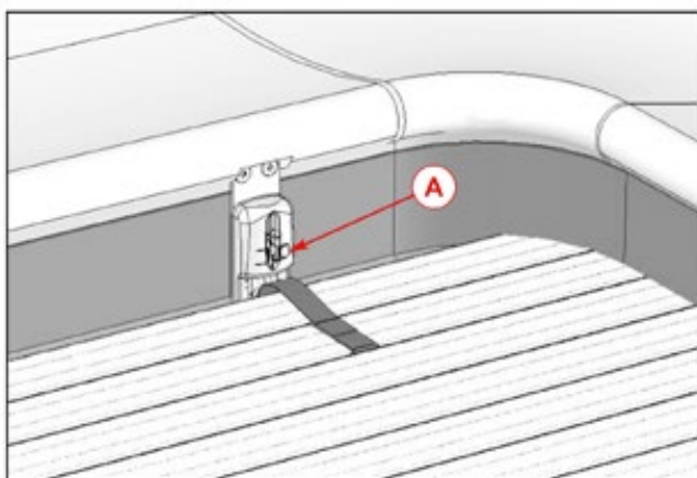
Figure 48 – Securing and releasing the cover apron
