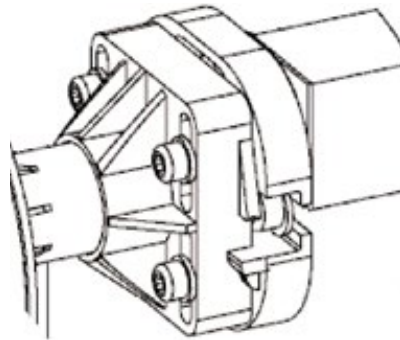
Figure 41 – Fitting the axle into the bearing mounting unit
