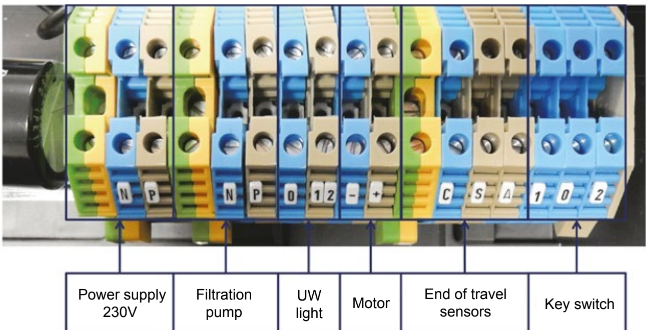
Figure 56 – XL URBAN POOL electrical panel
