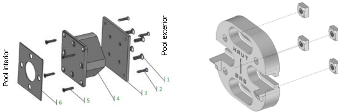
Figure 38 – Assembly of the bearing mounting unit
