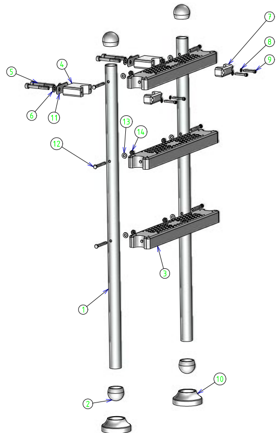
Figure 30 – Assembling the ladder
