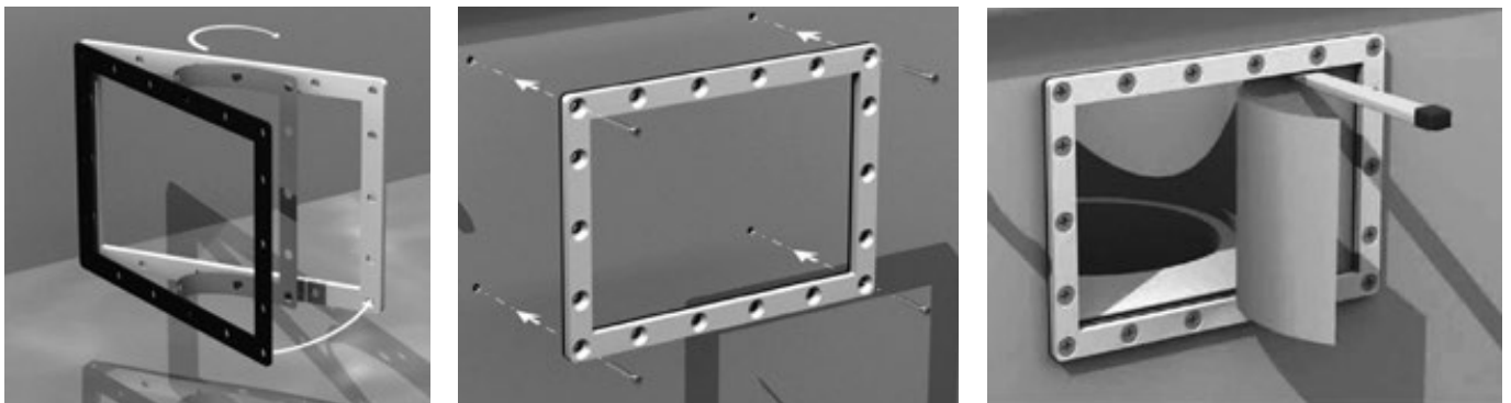
Figure 39 – Mounting the skimmer flange
