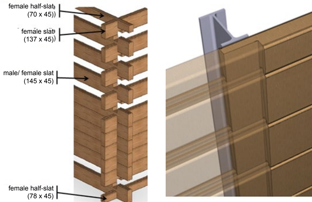
Figure 10 – Slotting together the wooden slats
