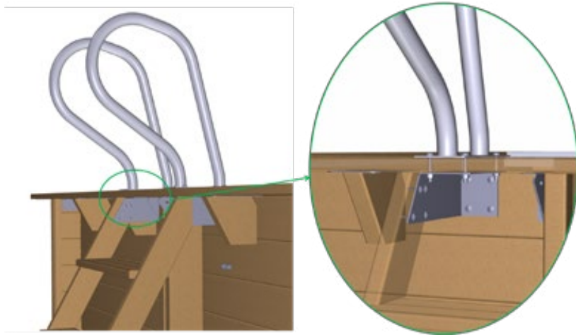
Figure 54 – Mounting the ladder hand rails
