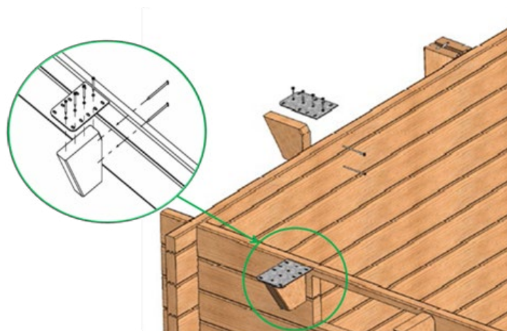
Figure 15 – Fastening metallic plates to the wooden corbels
