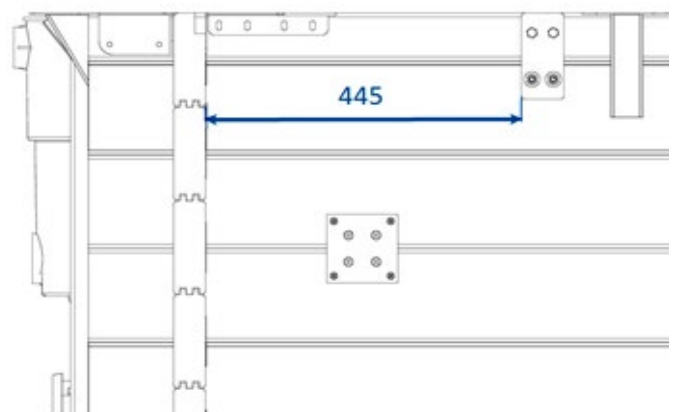
Figure 32 – Position of the beam mounting counter plate
